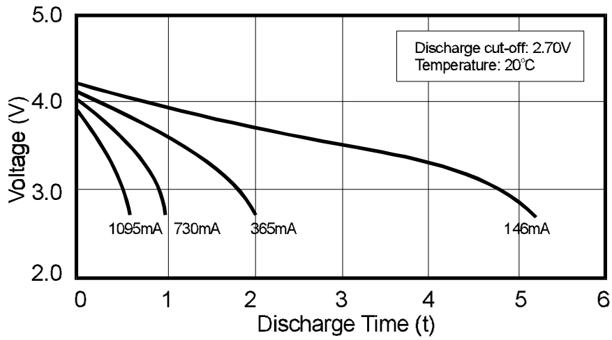
Figure 3: Voltage/Time discharge characteristics 600-0601
