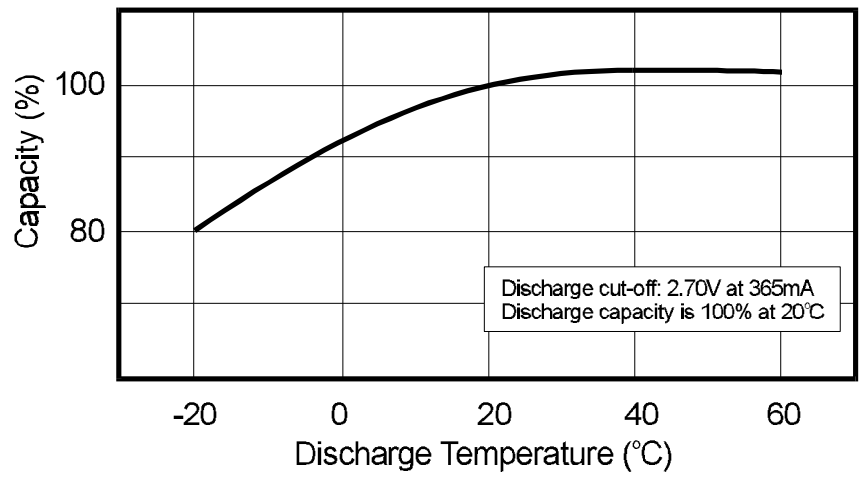
Figure 4: Capacity/Temperature discharge characteristics 600-0602
