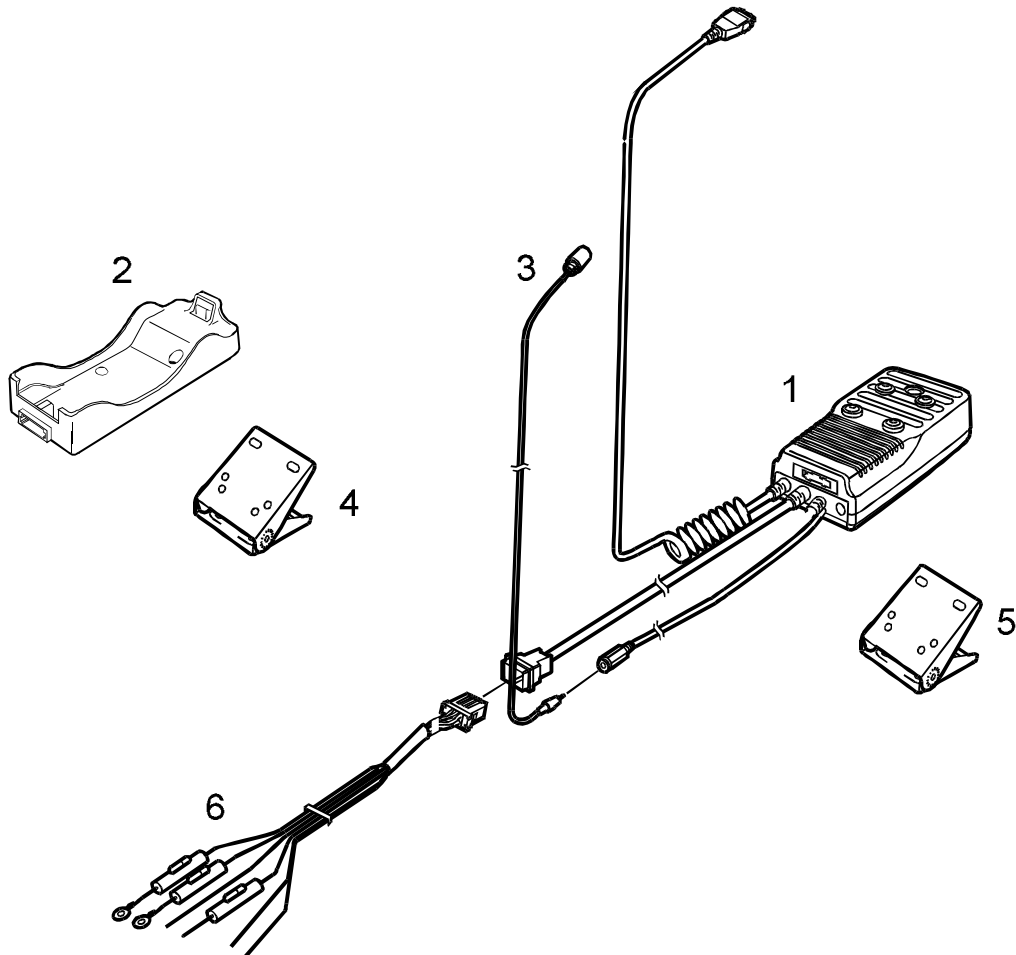
Figure 2: Handsfree Car Mount Kit 600-0202
