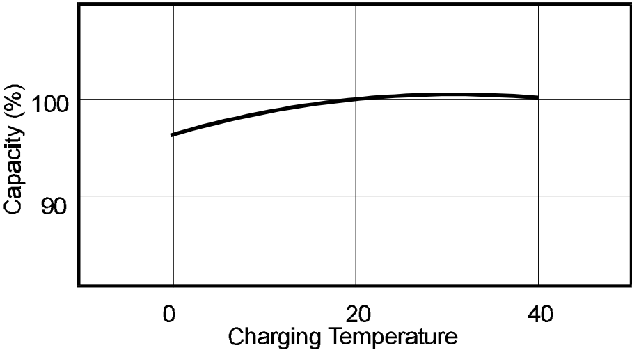
Figure 7: Capacity/Charging Temperature characteristics 600-0604
