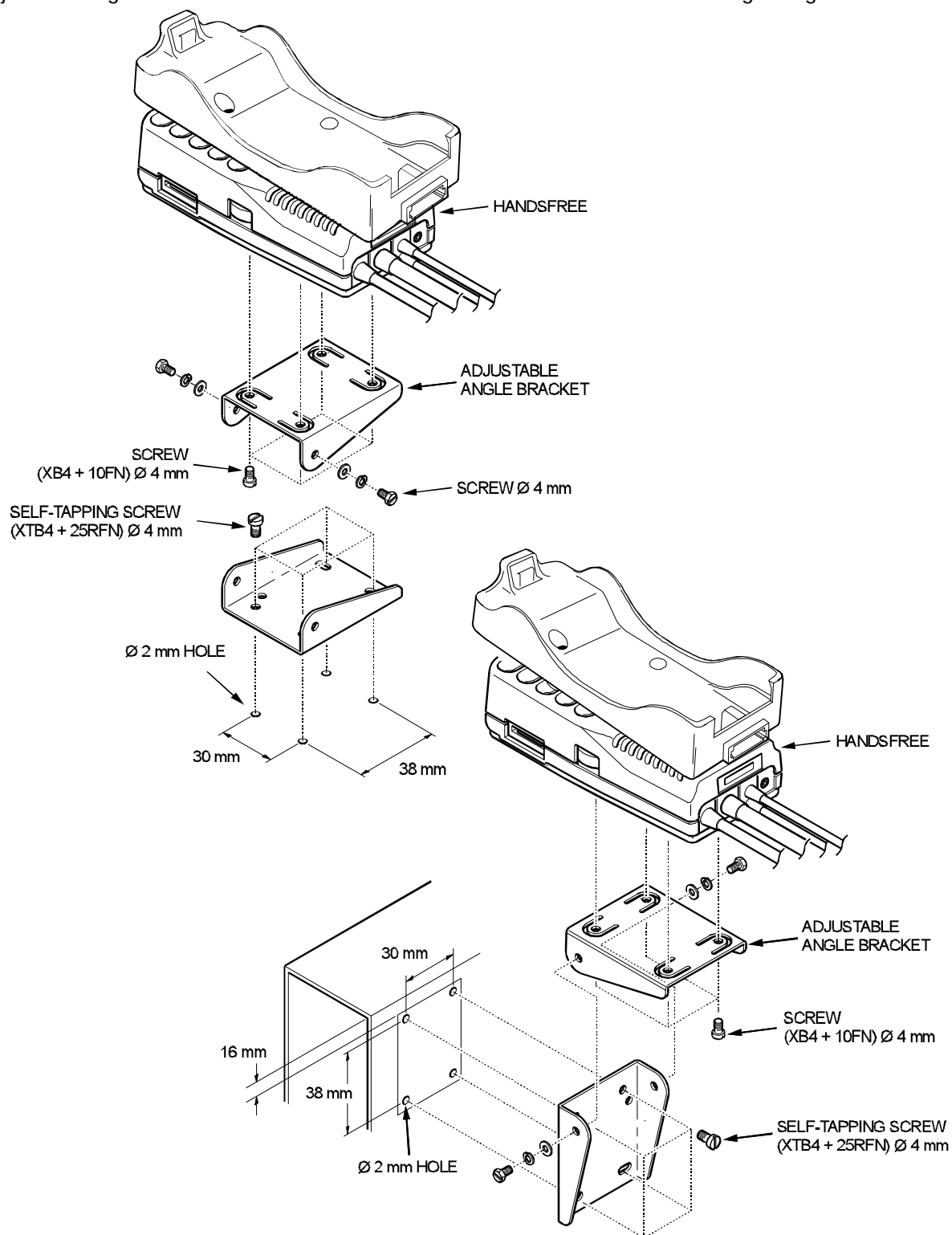
Figure 4: Adjustable angle bracket configurations
