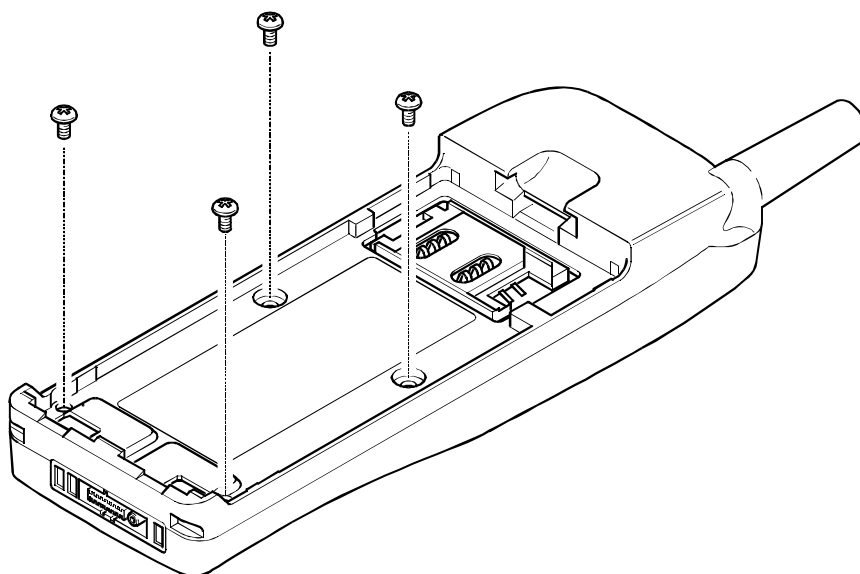
Figure 10: Case reassembly
