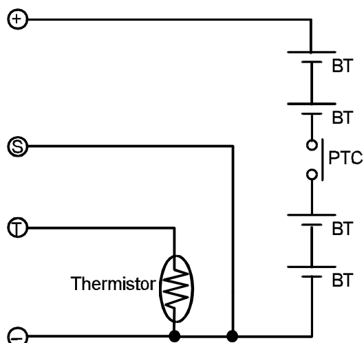
Figure 1: Circuit diagram of Ni-MH battery
