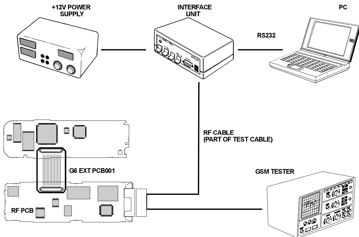
PCB TEST SETUP
