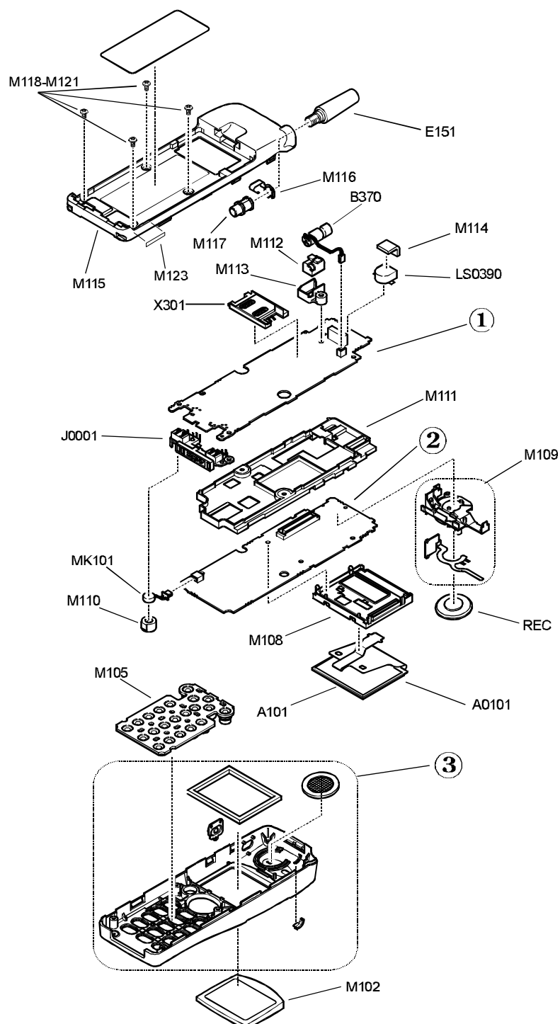
Figure 1: Handheld Unit
