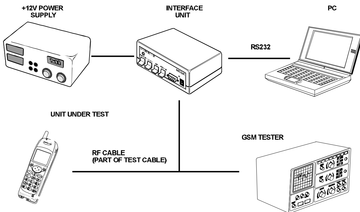
COMPLETE UNIT TEST SETUP
